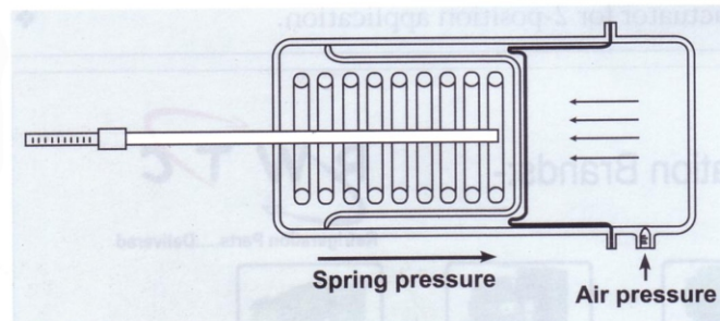
Figure 3: Pneumatic Actuator.
