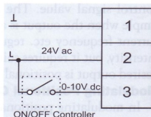
Figure 7 : 2-position operation of a modulating actuator.
