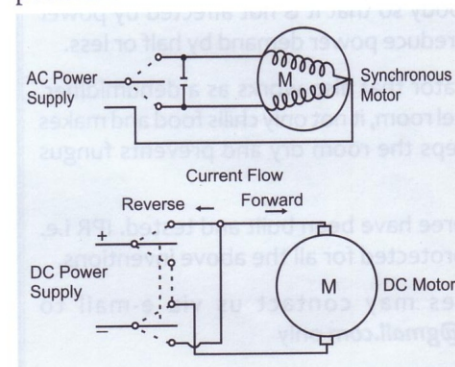
Figure 4 & 5: Internal connection details of synchronous motor
