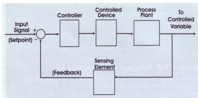
Figure 1 : Block Diagram of a Control Loop.
